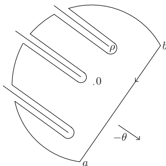
FIGURE 4.1. The contour \Gamma_R
