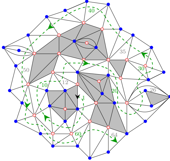
Figure 4: The exploration of the percolation interface of the example in Figure ?? until time \Theta . The interface is in green. The gray parts are the finite regions (free Boltzmann triangulations) discovered during the peeling process ( they are revealed respectively at steps 12, 26, 35, 50 and \Theta = 64 ).
