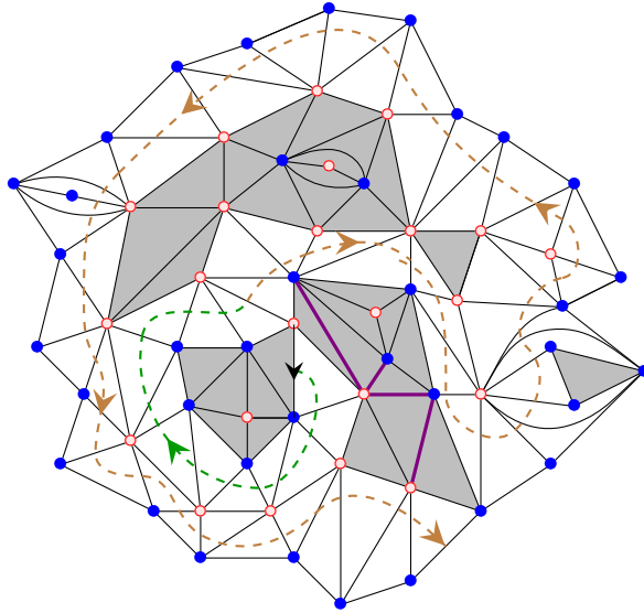
Figure 5: The exploration of the percolation interface of the example in Figure ?? until time \Theta . The interface until time \Delta is in green. The interface during time \Theta - \Delta is in brown. We add \mathbf{E} edges (in violet) that belong to the free Boltzmann triangulation discovered at step \Theta . Here, \Delta = 12 , \Theta = 64 and \mathbf{E} = 4 .
