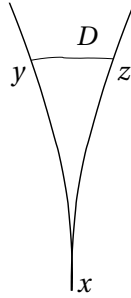
FIGURE 10. The coherence argument.
