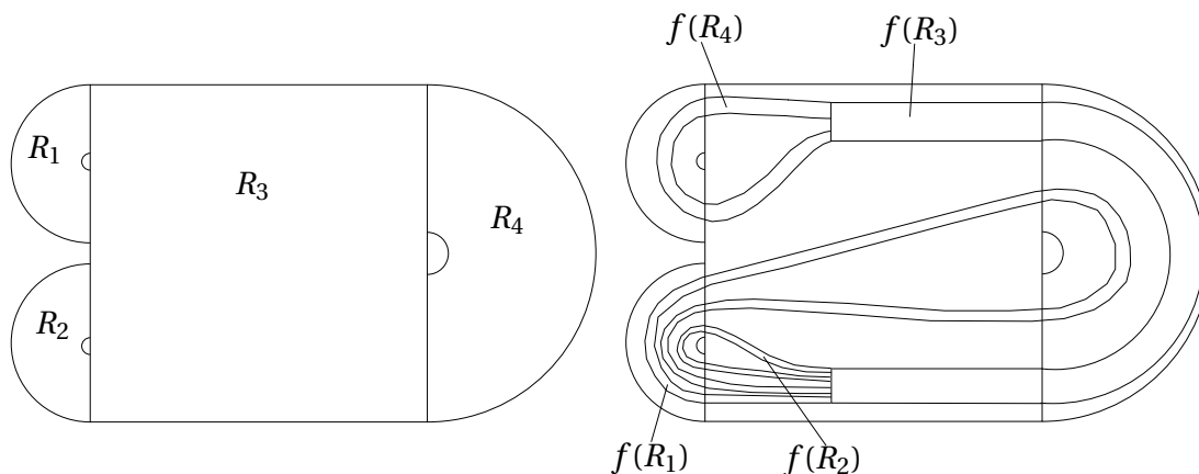
FIGURE 3. Construction of the Plykin attractor.
