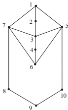
Figure: An example of regular strong bipartite partition with associated graph.
