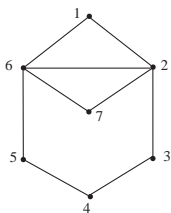
Figure: An example of regular strong nonbipartite partition with
