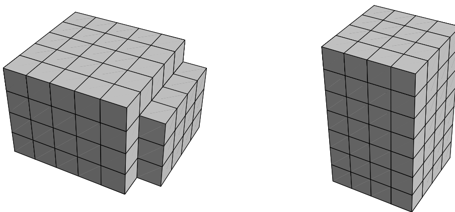
figure 3.17: polyominoes in \widetilde{\mathcal{M}}_{112} \setminus \mathcal{S}_{112}, \mathcal{M}_{112} \setminus \widetilde{\mathcal{M}}_{112} .
