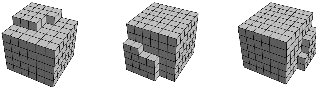
figure 3.15: the canonical polyominoes \mathfrak{m}_{194}, \mathfrak{m}_{230}, \mathfrak{m}_{266}
