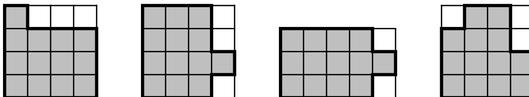
figure 2.15: elements of \{m_{13}\}, S_{13} \setminus \{m_{13}\}, \tilde{M}_{13} \setminus S_{13}, M_{13} \setminus \tilde{M}_{13}
