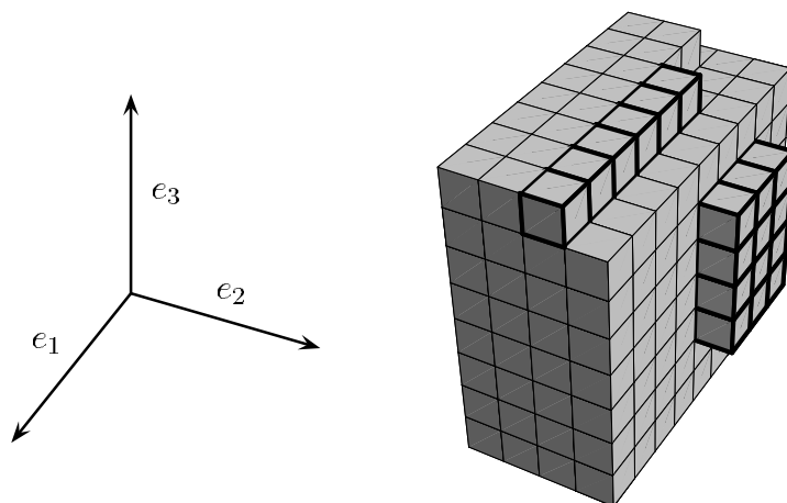
figure 3.4: the bar b_1(c, 2, 7) and the slice s_2(c, 4)
