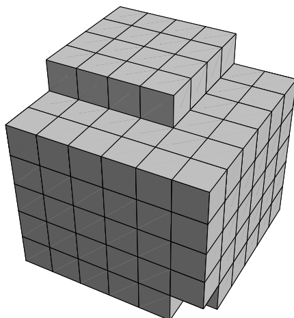
figure 3.18: an element of \mathcal{M}_{195}
