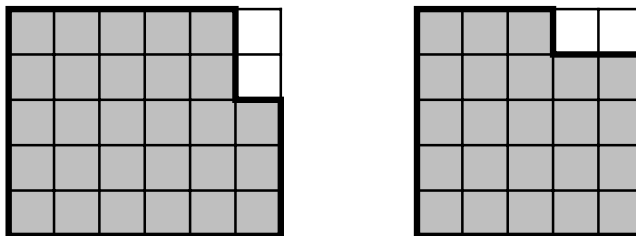
figure 2.14: the canonical polyominoes m_{28}, m_{23}
