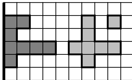
figure 2.9: horizontal projection p_1
