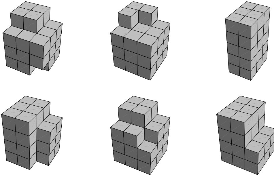
figure 3.3: some elements of \mathcal{M}_{30}
