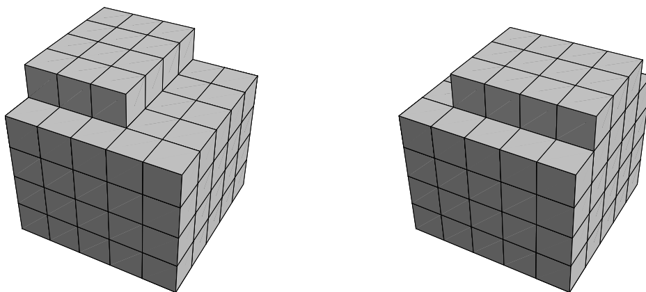
figure 3.16: polyominoes in \{\mathbf{m}_{112}\}, \mathcal{S}_{112} \setminus \{\mathbf{m}_{112}\} .
